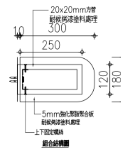
⑤ A4 懸臂式服務空間標示 Size:300x180x30mm
