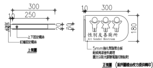
⑤ A4 懸臂式服務空間標示 Size:300x180x30mm
